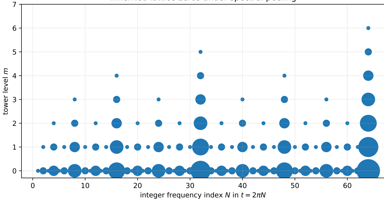
Inherited lattice zeros under spectral peeling
