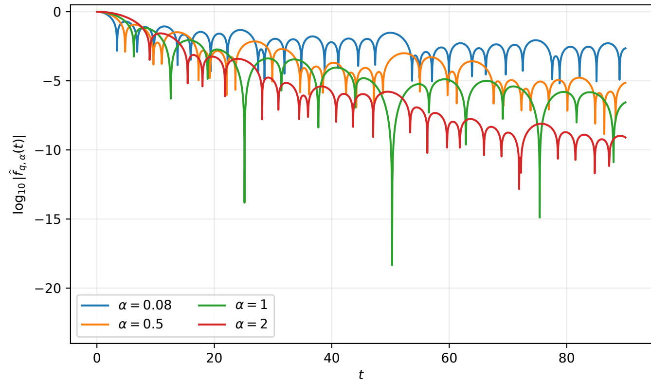
Geometric Bessel products at q = 1/2
