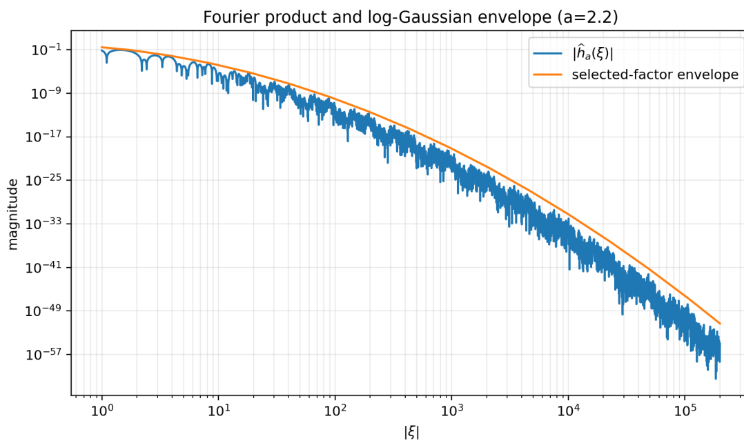
Figure 31: The Fourier product for a = 2.2 and the selected-factor bound (17.1). The oscillatory zeros sit well below the envelope, while the quadratic decay in \log |\xi| is clearly visible.
