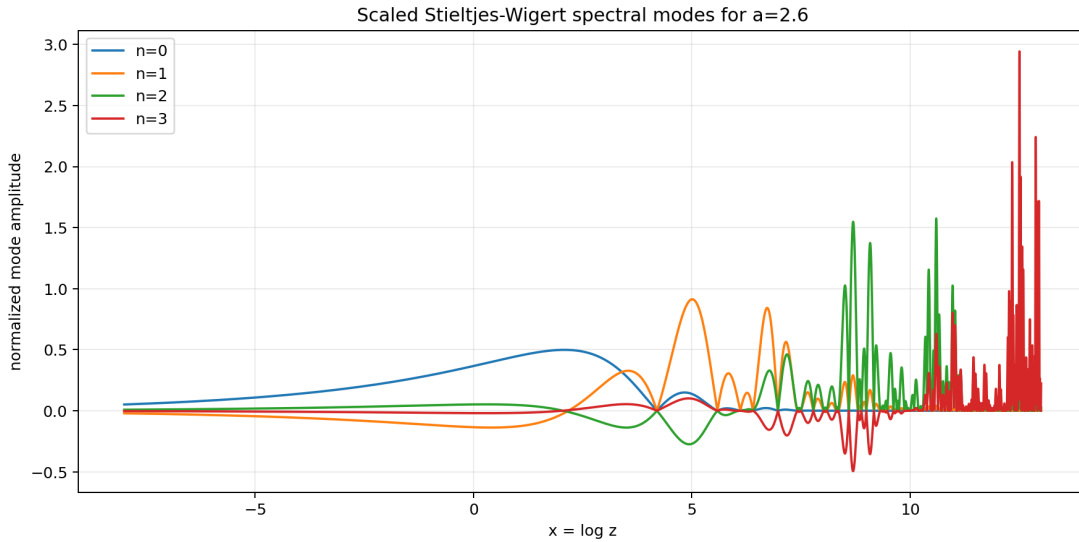
Figure 25: The first four normalized spectral modes P_{a,n}(t^2)\widehat{h_a}(t) of the differential ladder at a = 2.6 , displayed against \log(t^2) ( theorem 13.12 ). Their numerical Gram matrix is the identity to the precision recorded in the package's orthogonal_ladder_validation_a_2_6.csv .
