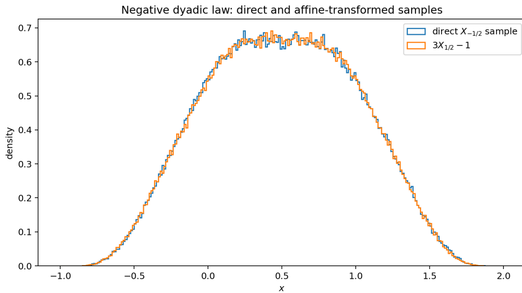
Figure 39: Independent simulations of X_{-1/2} and 3X_{1/2} - 1 . The visual agreement supplements the exact digit-reflection coupling in table 22 .
