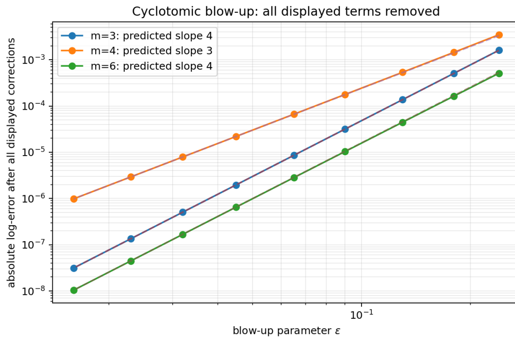
Figure 43: Absolute logarithmic error after removing the limit, all subcritical terms, and the complete order- \varepsilon^d layer. The predicted next exponents are d + 1 : four for m = 3, 6 and three for m = 4 .
