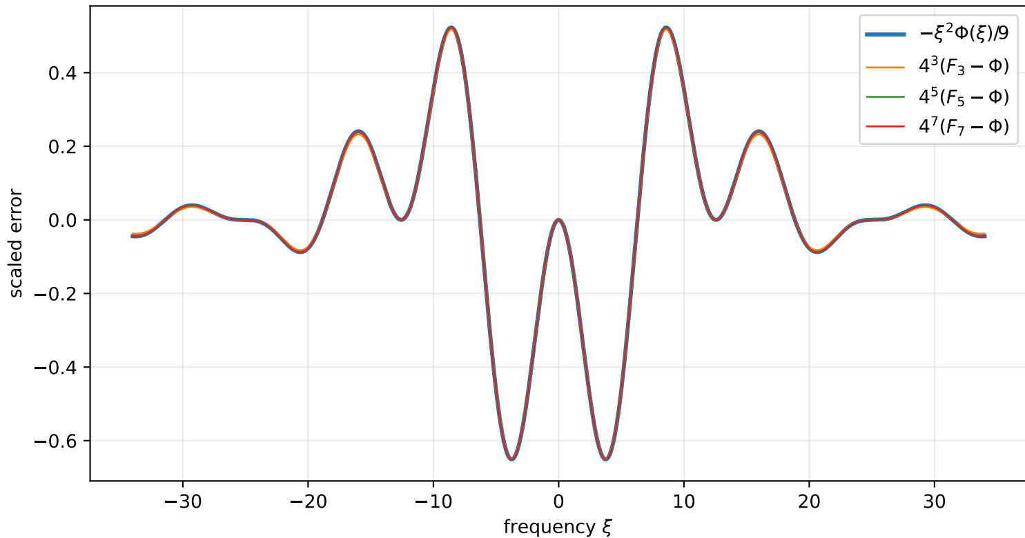
Weighted L^p limit profile of the Fourier error
