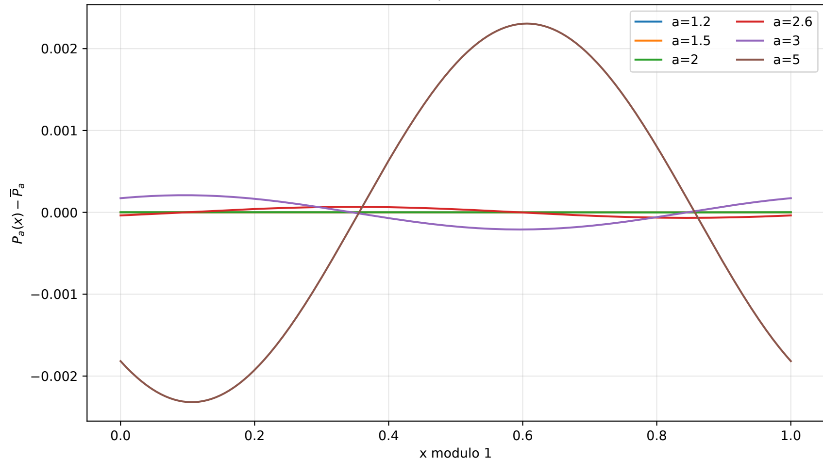
General-base periodic correction
