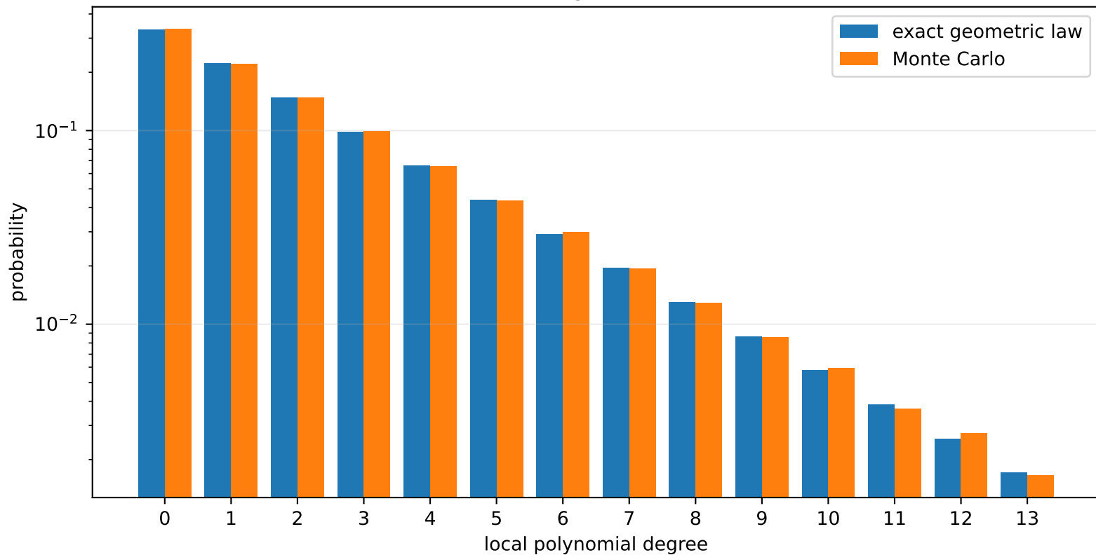
Local degree for a=3
