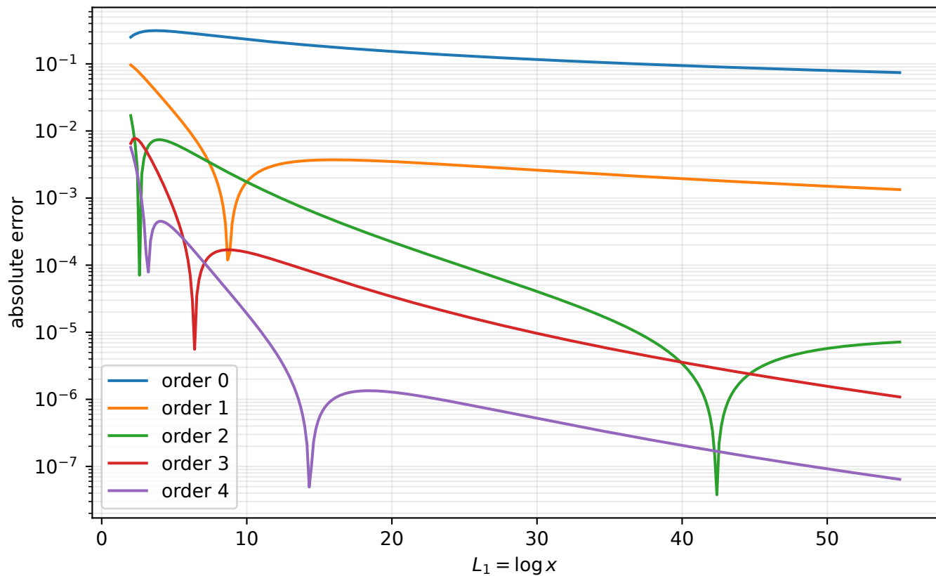
Logarithmic asymptotics for W_0(x)
