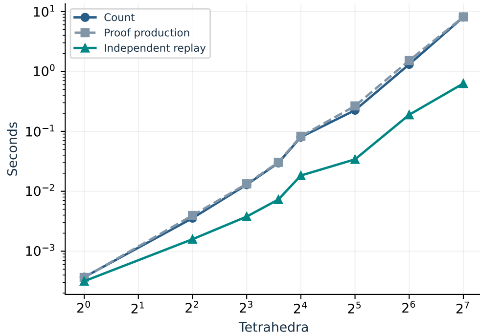
Full native topology query
