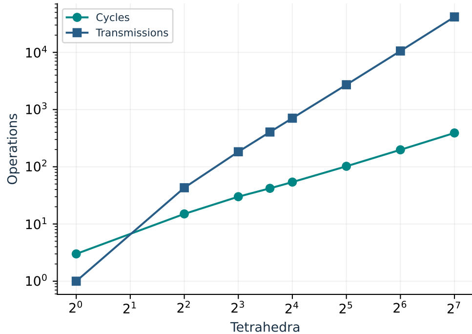
Ordinary component query
