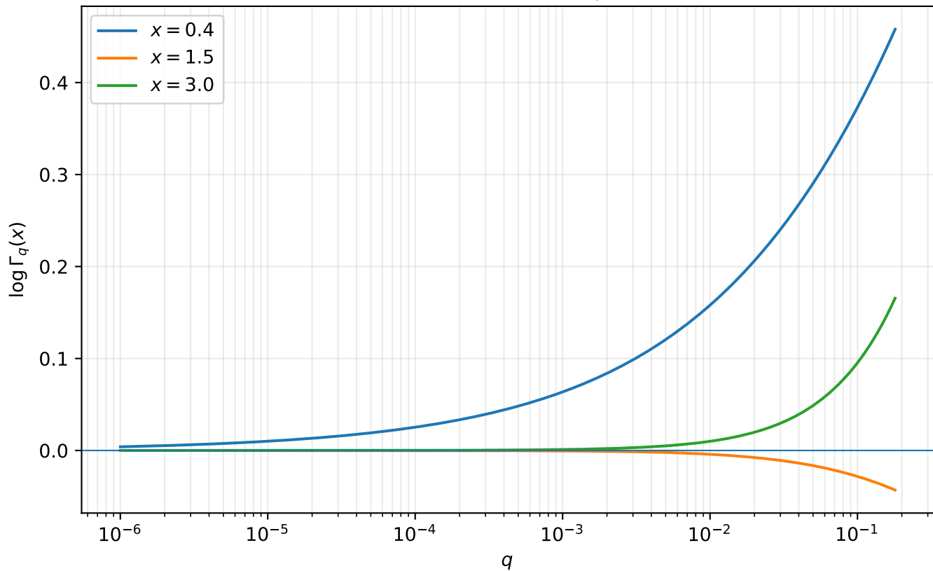
Newton-polygon regimes of \Gamma_q(x) near q = 0
