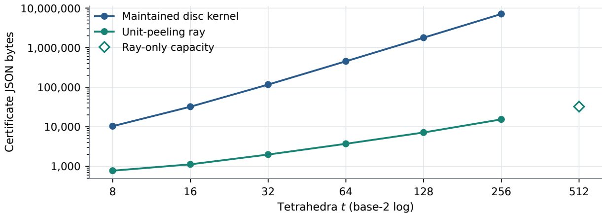
Essential-disc certificates: retained exact sizes
