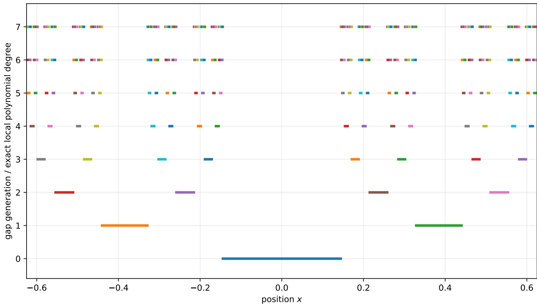
Complementary gaps of K_a for a = 2.6
