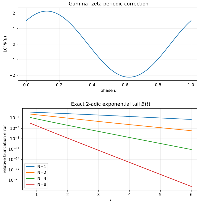
Figure 4: Top: the centered Gamma-zeta fluctuation \Psi – tiny amplitude, same asymptotic order as the constants. Bottom: relative error of N = 1, 2, 4, 8 terms of the exact 2-adic series for B(t) , with the elementary enclosure of theorem T.2 .
