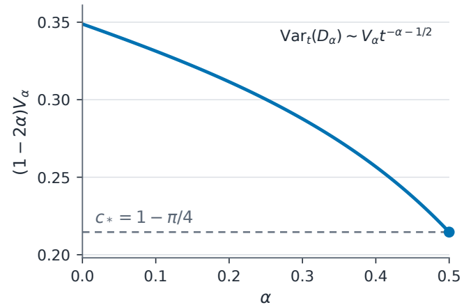
(a) Approach to the critical pole
