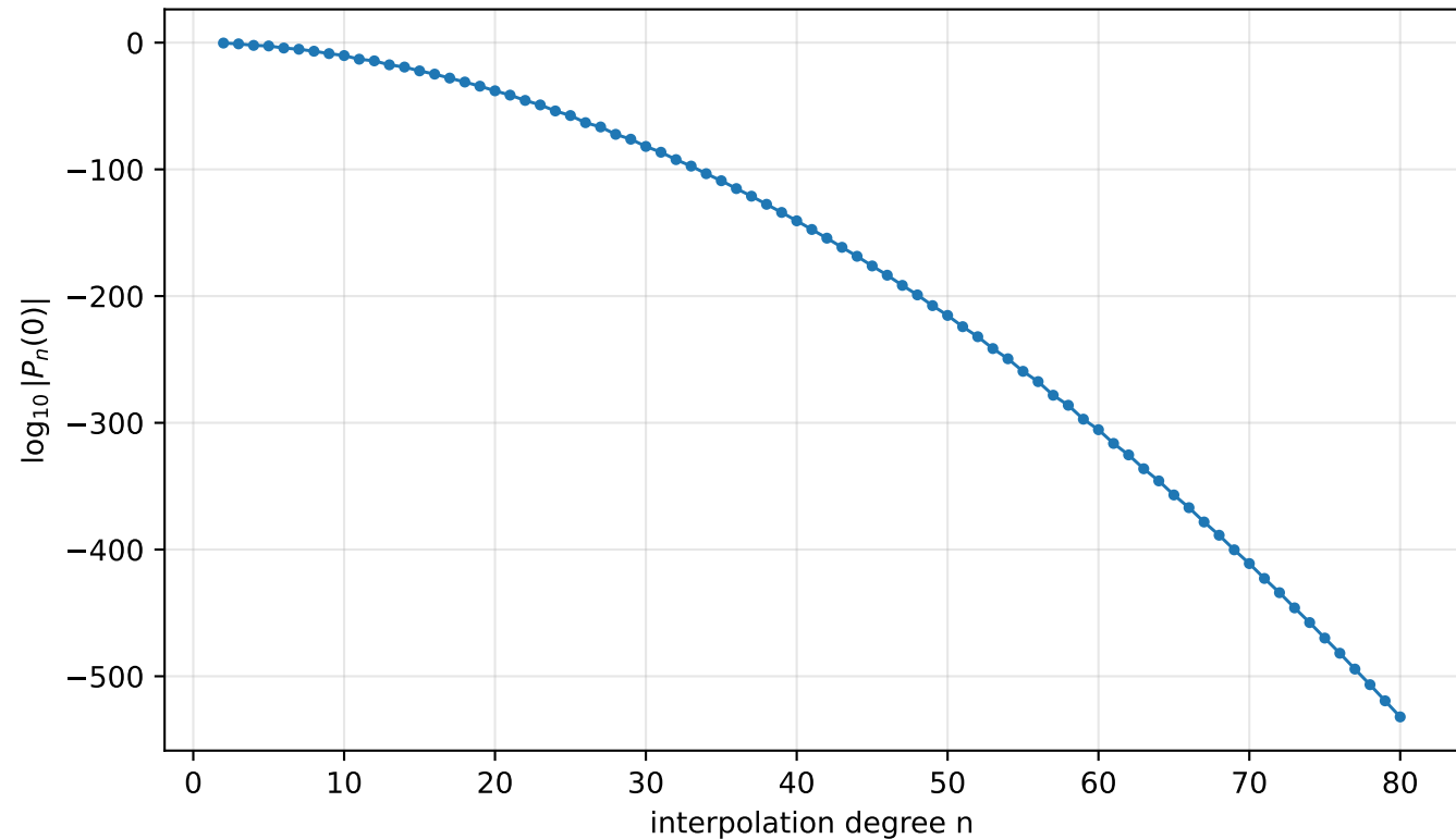
Fabius geometric-comb extrapolation at the accumulation point
