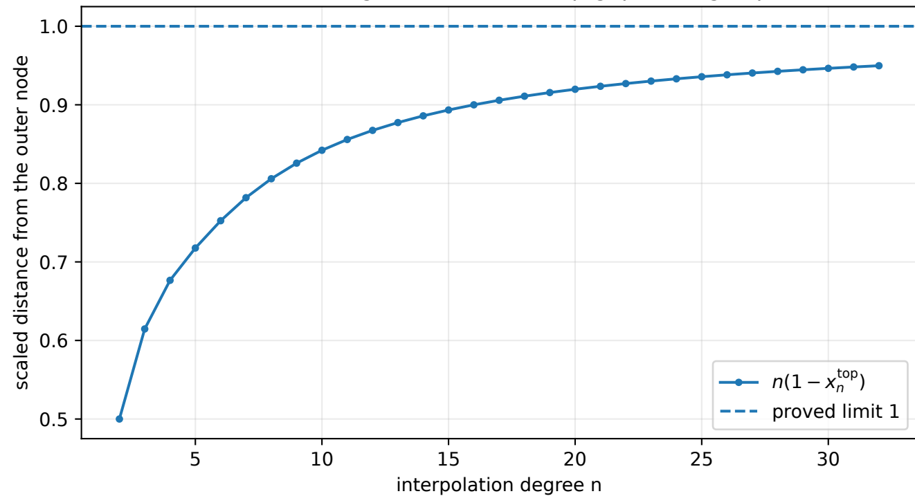
Location of the geometric-comb top-gap Lebesgue peak
