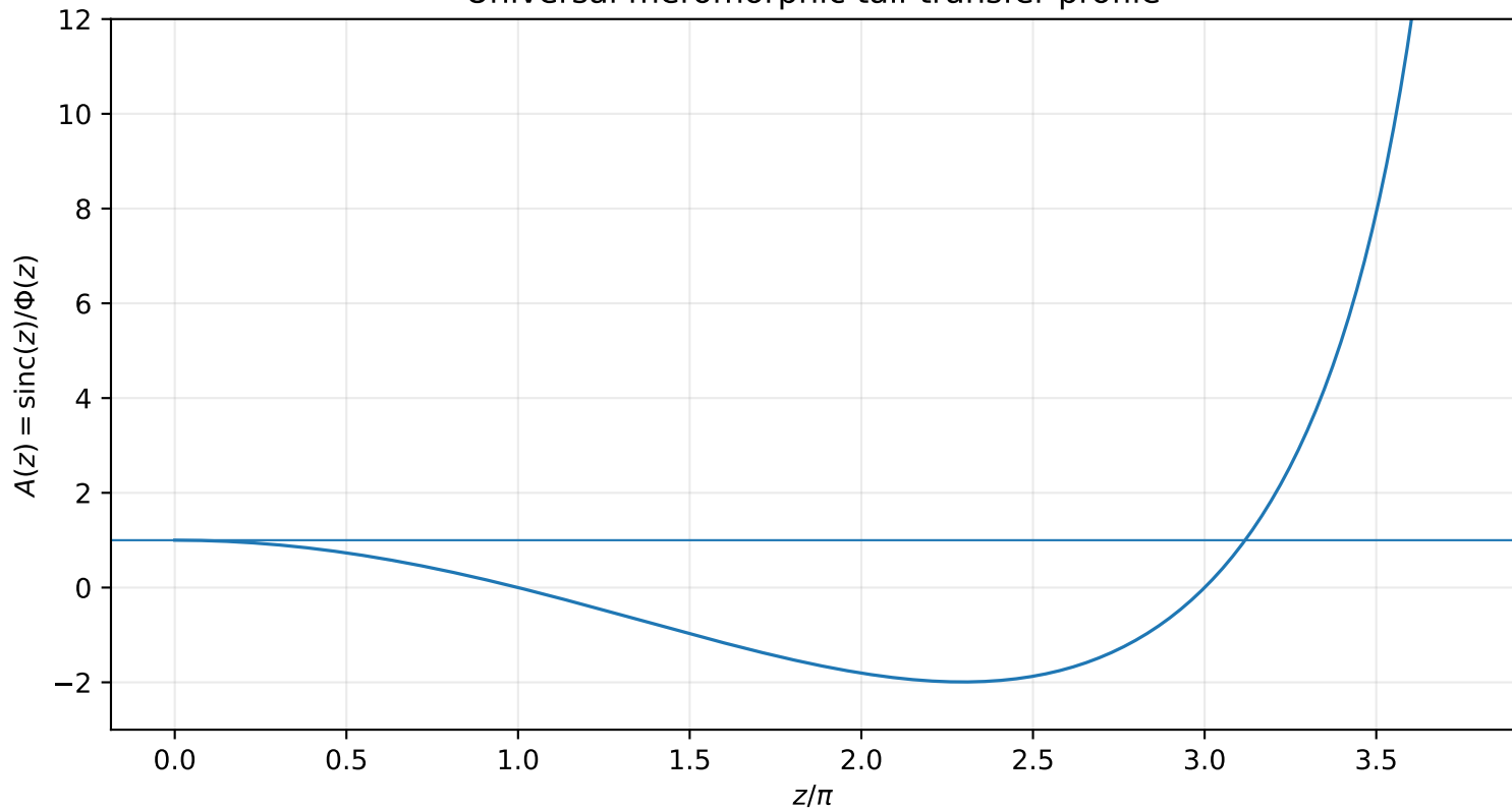
Universal meromorphic tail-transfer profile
