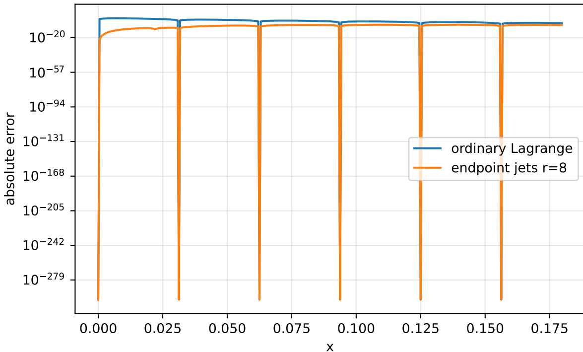
Left-endpoint error profile at N=32
