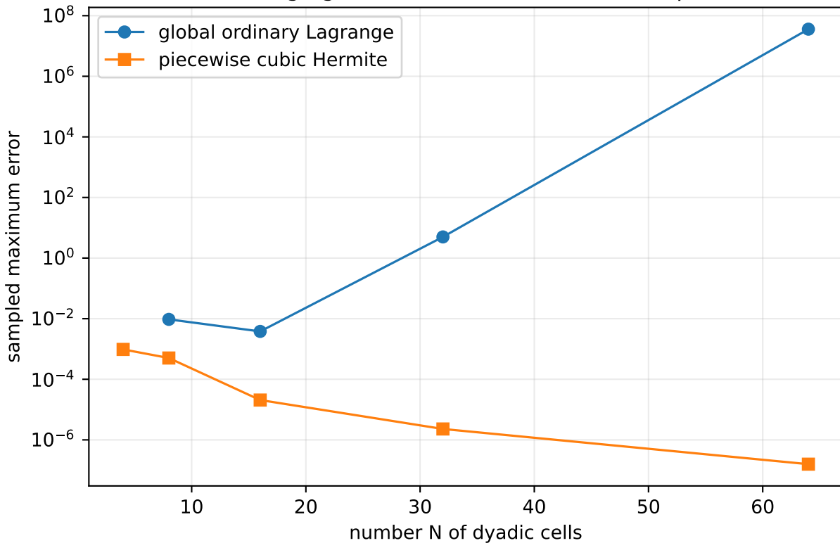
Global Runge growth versus stable local interpolation
