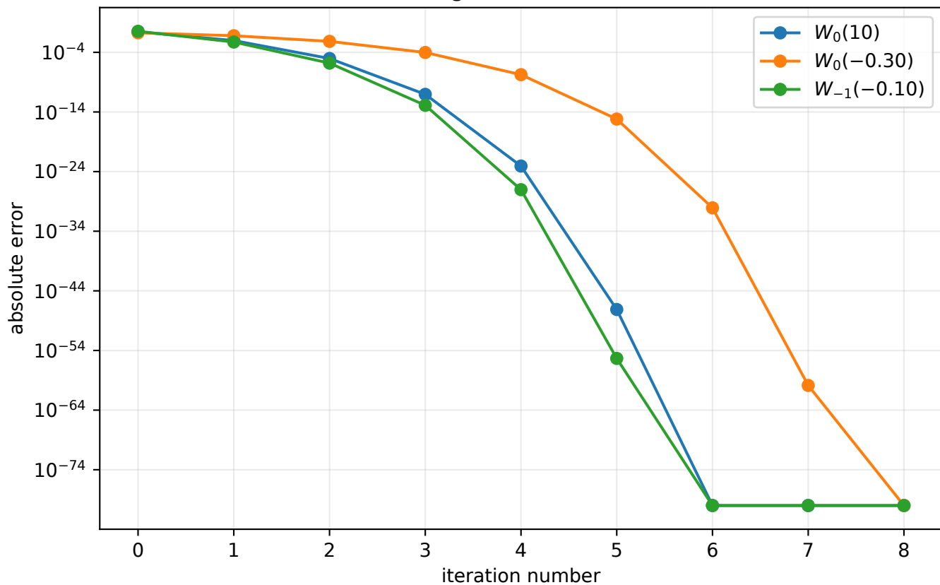
Branch-safe logarithmic Newton iteration
