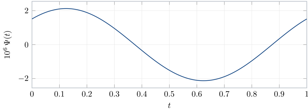
Figure 1: The periodic correction \Psi , magnified by 10^6 . The curve is indistinguishable from its first Fourier harmonic at this resolution, and the half-period antisymmetry \Psi(t + \frac{1}{2}) \approx -\Psi(t) visible here is the statement that the even harmonics are negligible. The vertical scale is the point of the picture: the oscillation is a few parts in a million in the logarithm, but it does not tend to zero.
