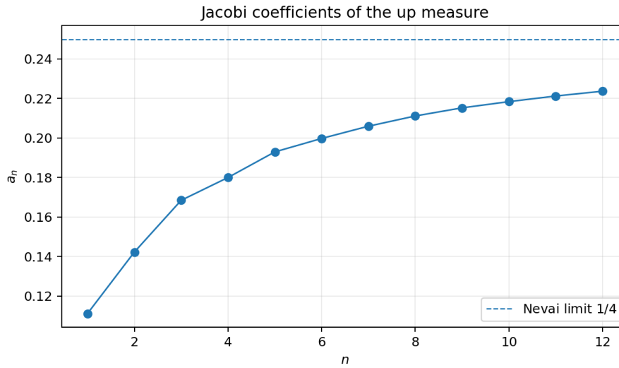
Figure 6: The first twelve exact Jacobi coefficients (shown in decimal form) and the rigorous limiting value 1/4 . Monotonicity is suggested but not proved.
