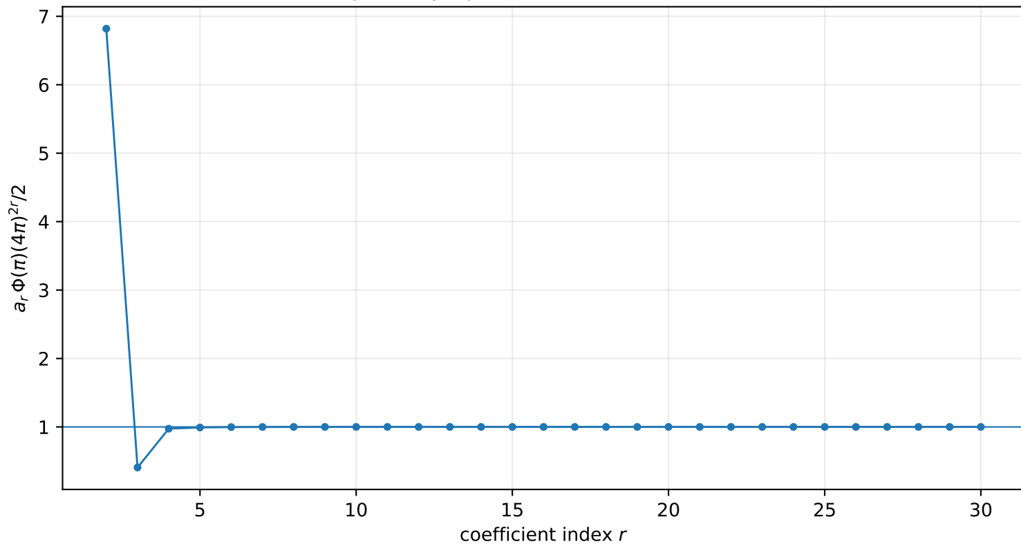
Nearest-pole asymptotic of the transfer coefficients
