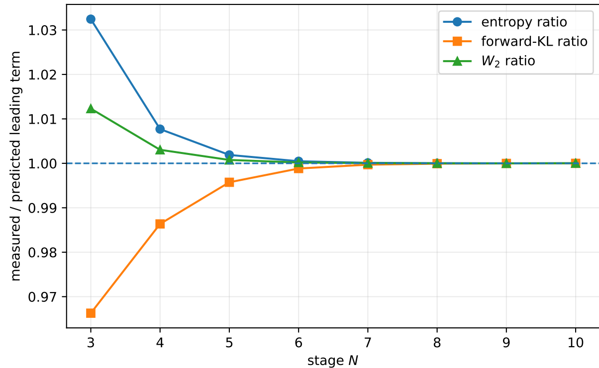
Information and finite- p transport asymptotics
