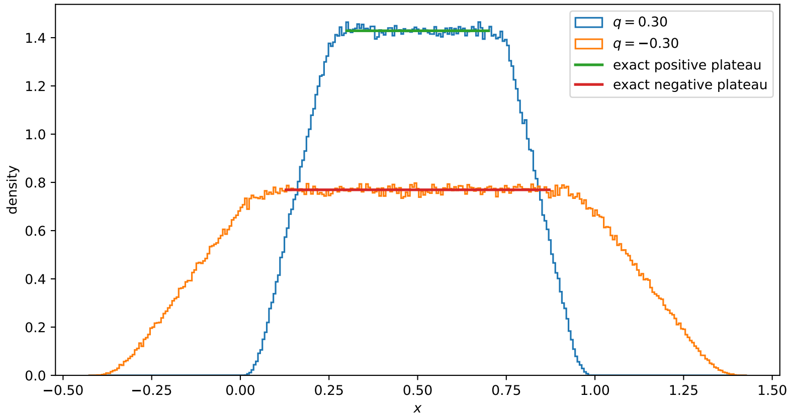
Dominant-digit plateaux and affine transport
