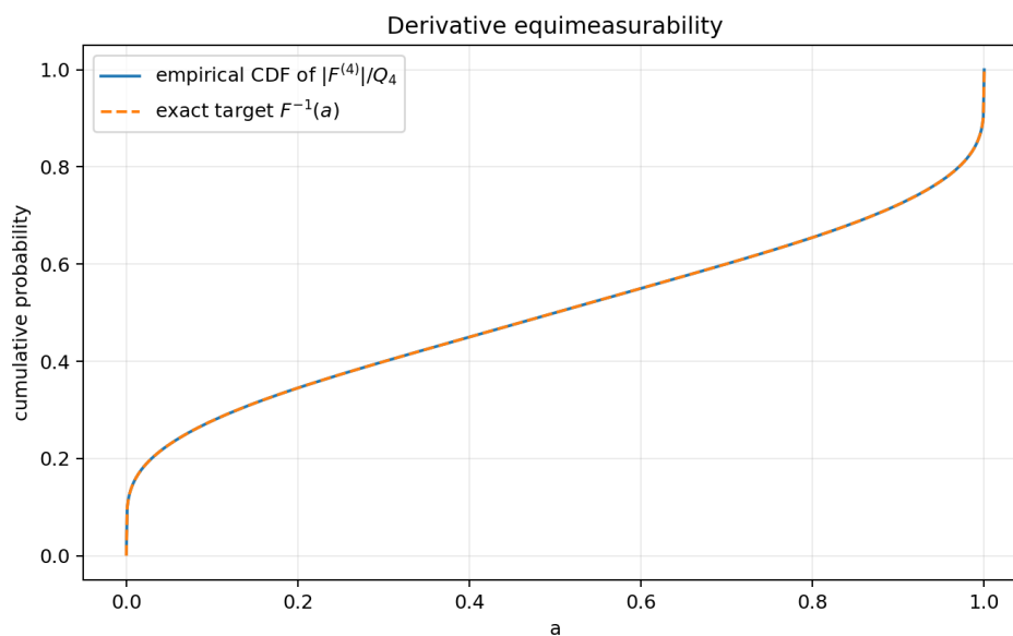
Figure 2: The empirical CDF of |F^{(4)}|/Q_4 lies on the exact target I = F^{-1} , illustrating theorem K.1 .
