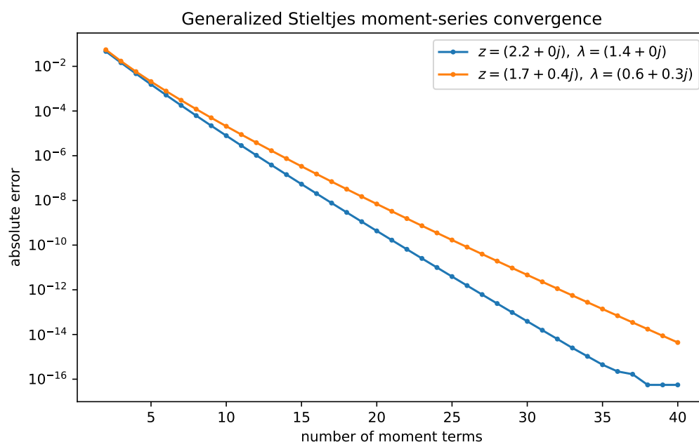
Figure 12: Convergence of the exact-moment expansion (1494) at two real/complex parameter pairs.
