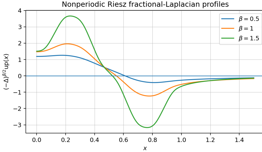
Figure 10: Nonperiodic singular-integral profiles of (-\Delta)^{\beta/2} up for three representative orders. Each profile has one positive zero in the plotted half-axis, motivating Conjecture N.4.
