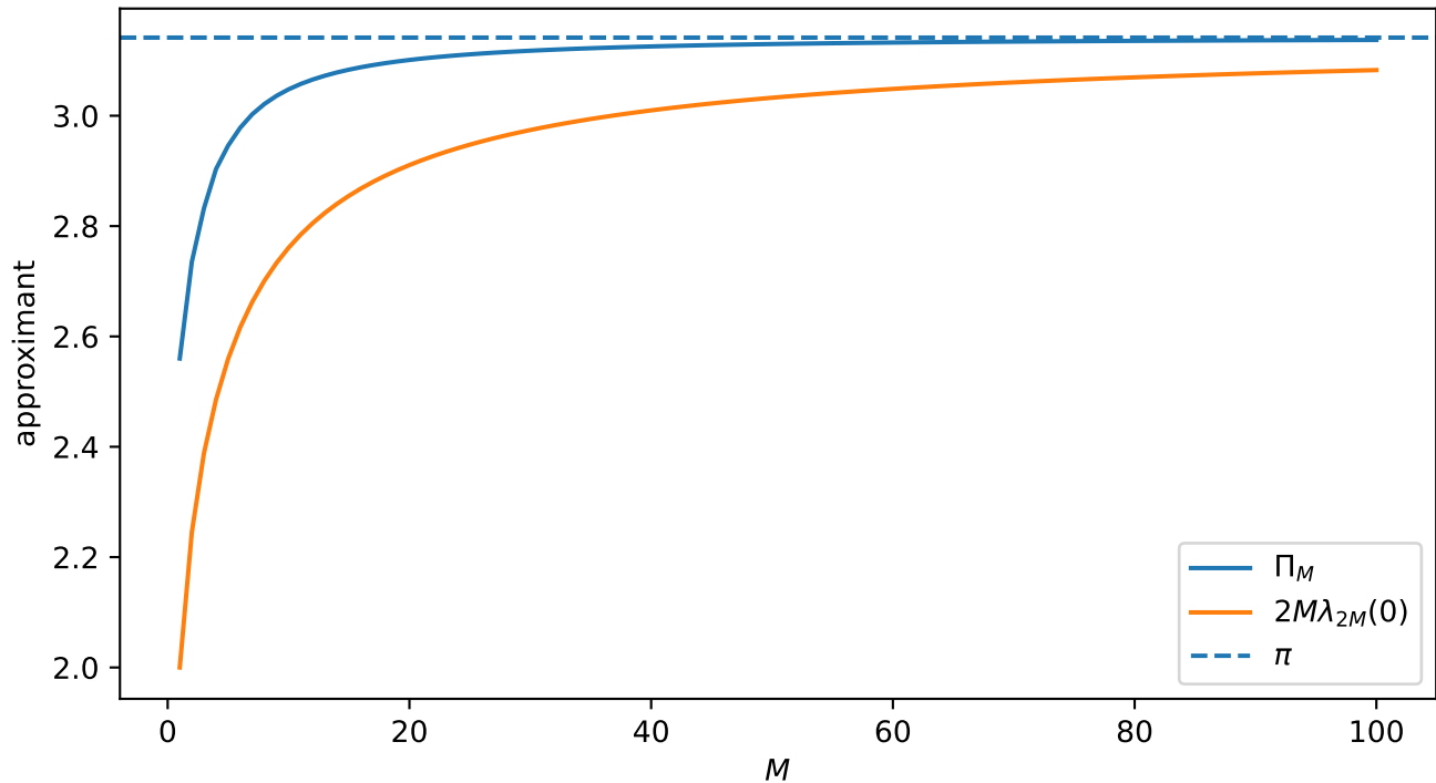
Two moment-theoretic approximations to pi
