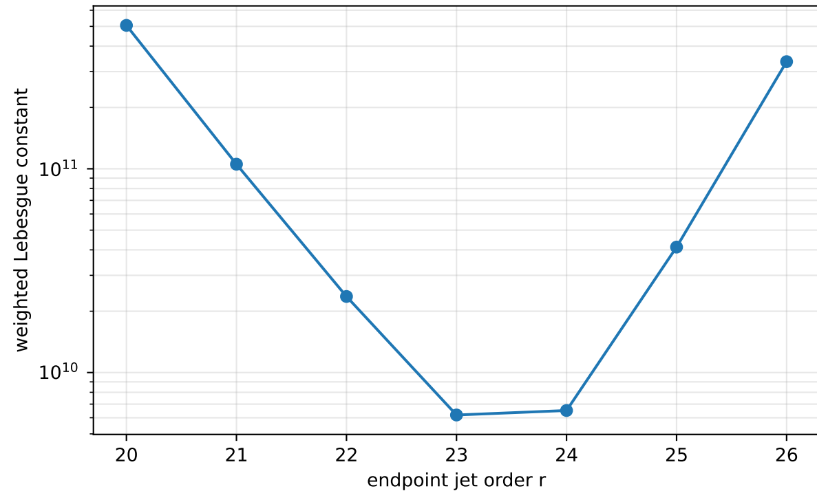
Endpoint-jet operator conditioning, N=128
