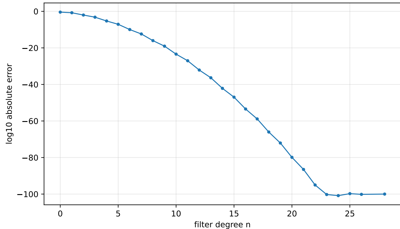
Reciprocal Rvachev sinc product from the q = 1/2 Lagrange filter
