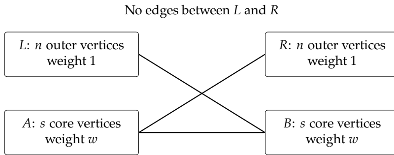
Figure 6: Each drawn connection denotes all edges between the indicated blocks. The core is a vertex cover of size 2s .
