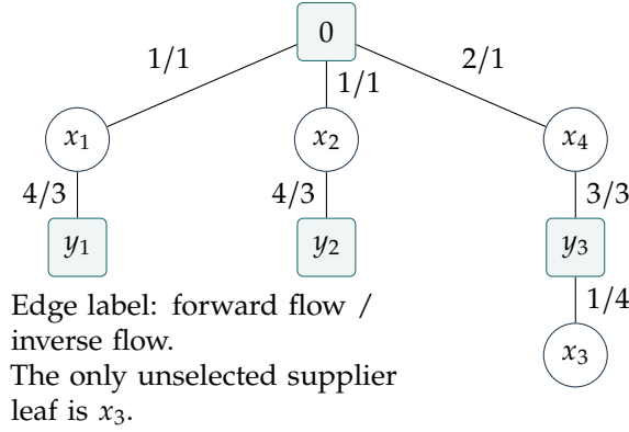
Figure 5: The common tree. Edges are drawn as undirected tree edges; transportation flow always goes from a supplier to a receiver.
