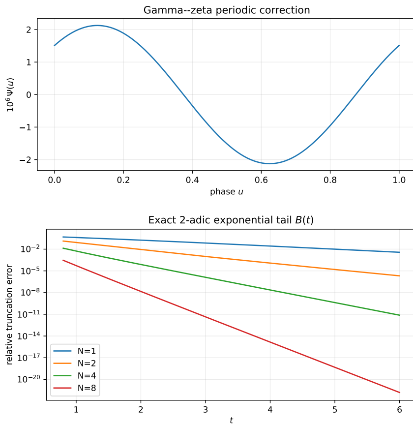
Figure 3: Top: the centered Gamma-zeta fluctuation \Psi – tiny amplitude, same asymptotic order as the constants. Bottom: relative error of N = 1, 2, 4, 8 terms of the exact 2-adic series for B(t) , with the elementary enclosure of theorem 10.2 .
