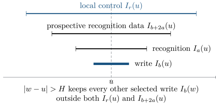
Figure 8: Read and write roles at an isolated anchor. The schematic shows the compiler regime r \geq b + 2a ; the abstract theorem allows either order. The separation conditions are H \geq b + r and H \geq 2b + 2a . Isolation itself reads I_{H+a}(u) .
