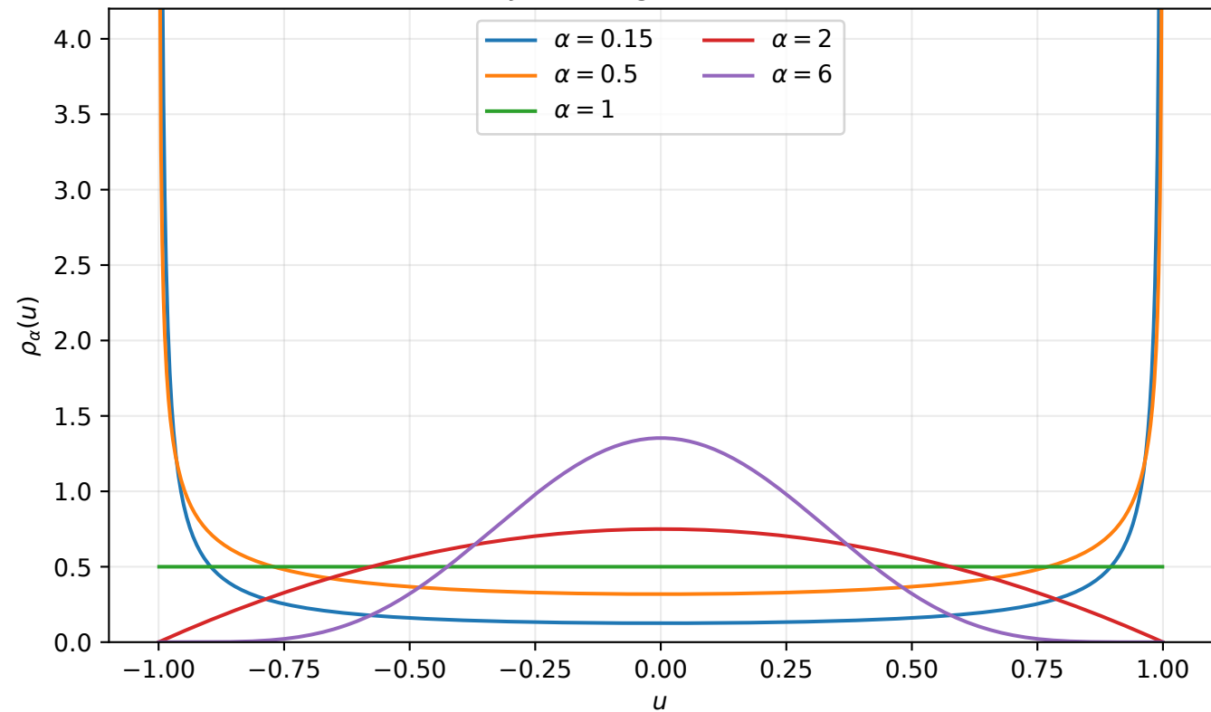
Jacobi digit densities
