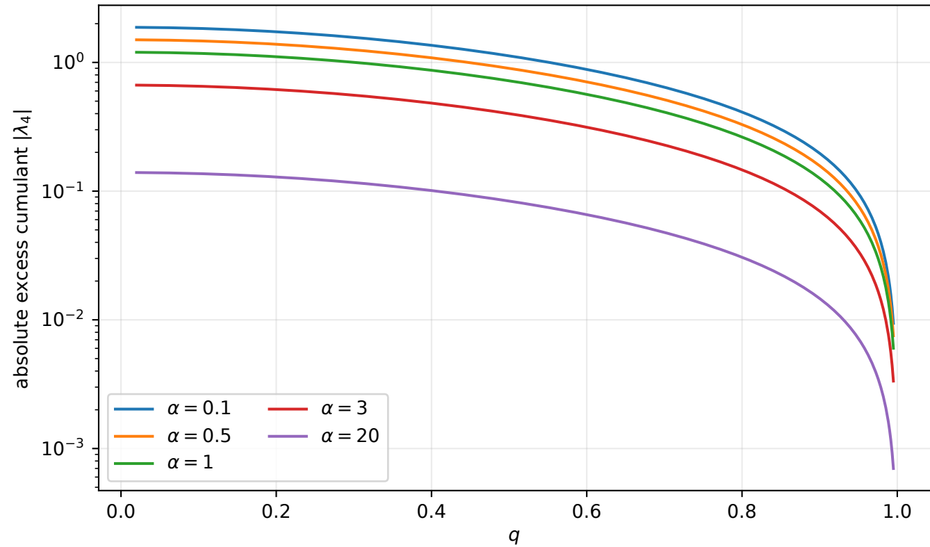
Two-parameter Gaussian corner: either q approaches 1 or \alpha grows
