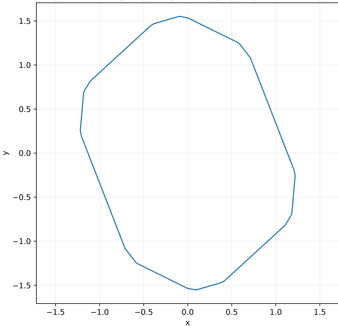
Eighteen-stage rotating zonotope
