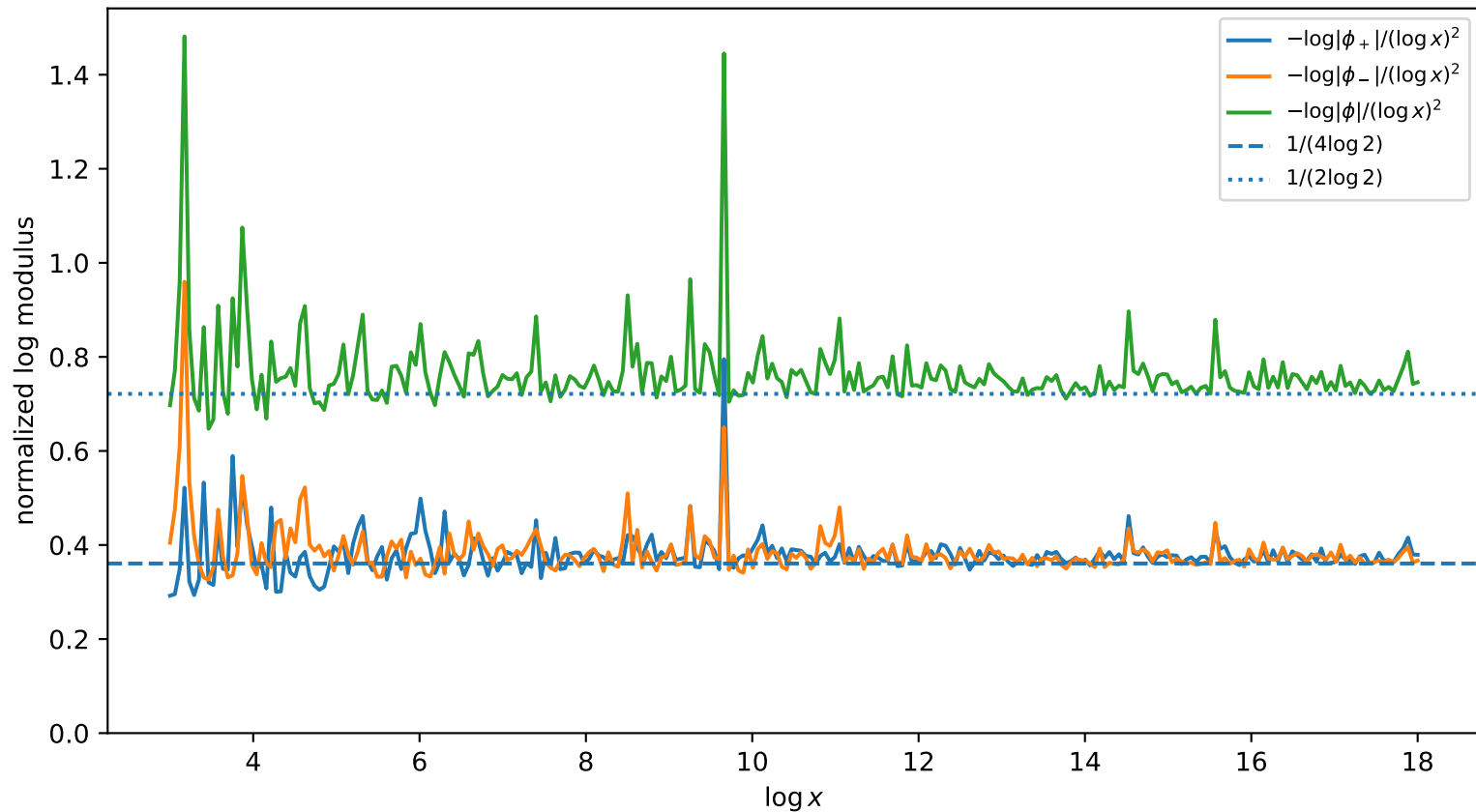
Quadratic-log Fourier decay along a nonresonant ray
