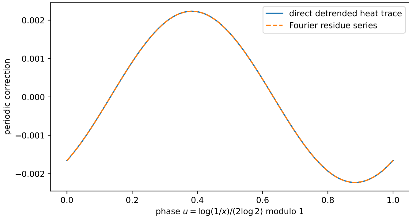
Dyadic heat trace: log-periodic correction
