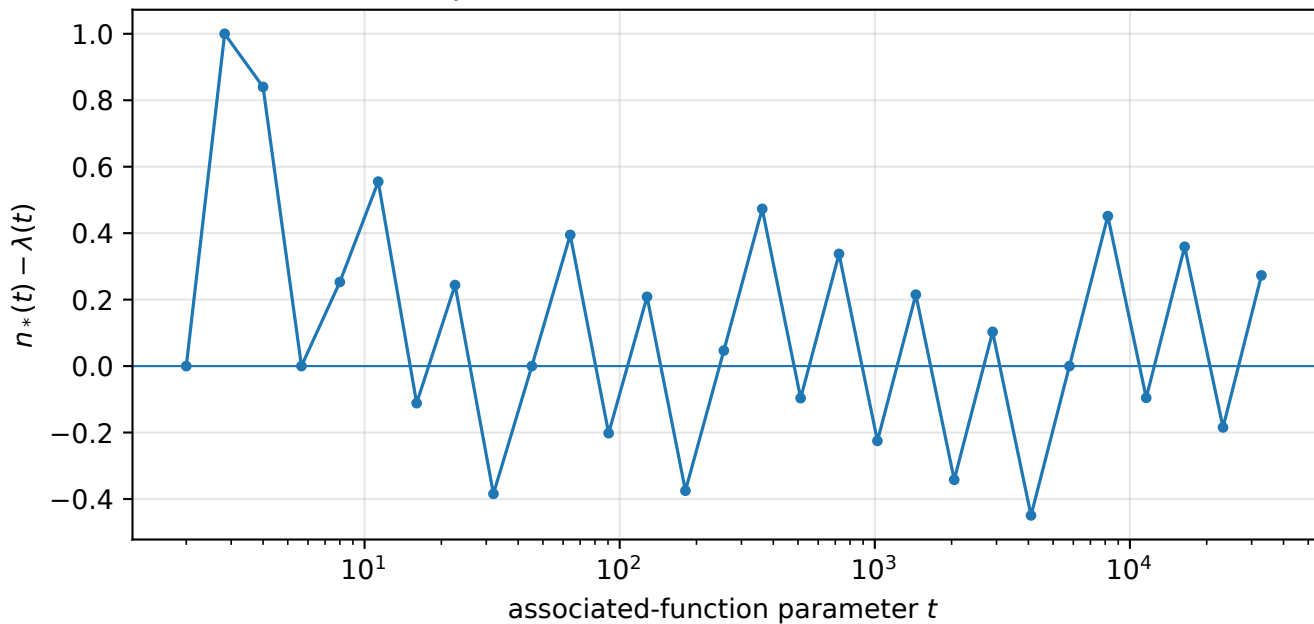
Lambert-W predictor for the normalized Carleman saddle
