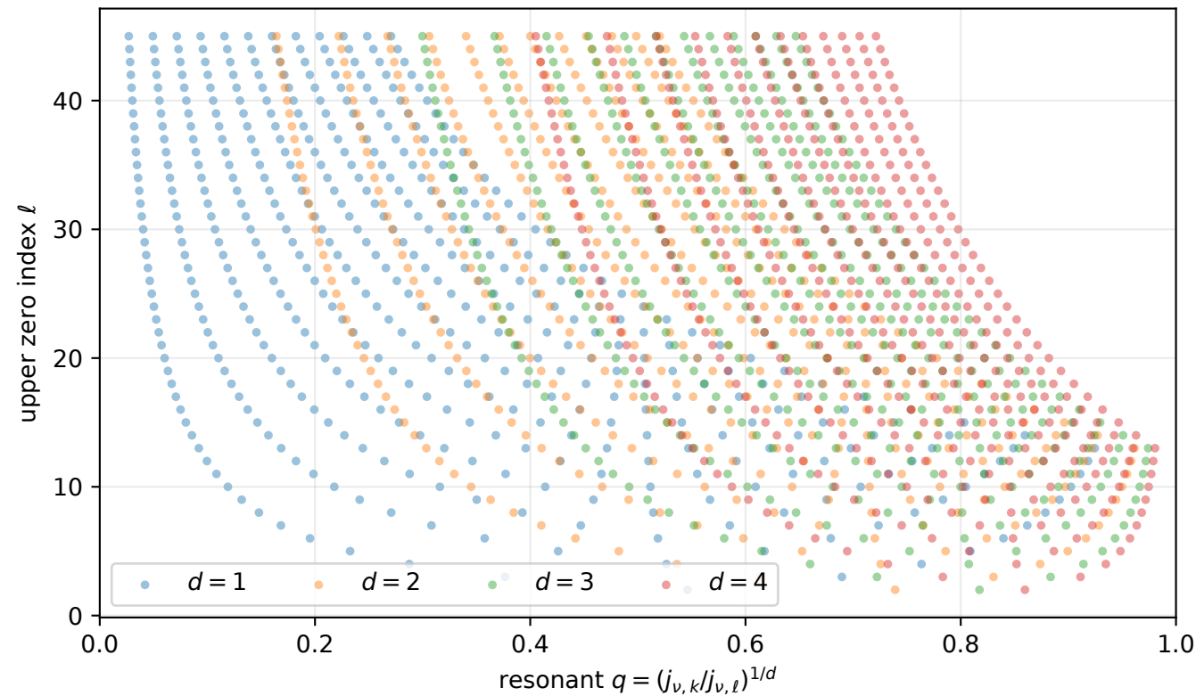
Countable-dense Bessel-scale resonances ( \alpha = 3/2 , \nu = 1 )
