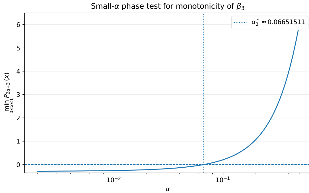
Figure 10: Minimum of the exact derivative-controlling polynomial P_{2\alpha+3} over 0 \leq q^2 \leq 1 . The zero crossing identifies the candidate threshold \alpha_3^* .
