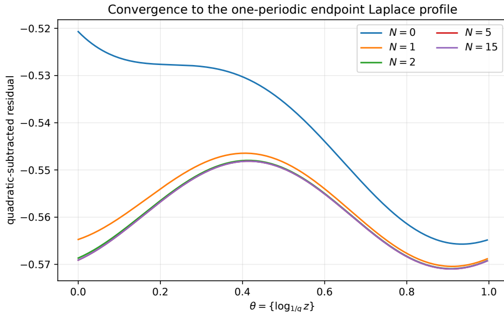
Figure 4: After subtraction of the quadratic and linear terms in (57), successive logarithmic decades converge rapidly to the same one-periodic profile. The plotted parameters are \alpha = 1.3 , q = 0.1 .
