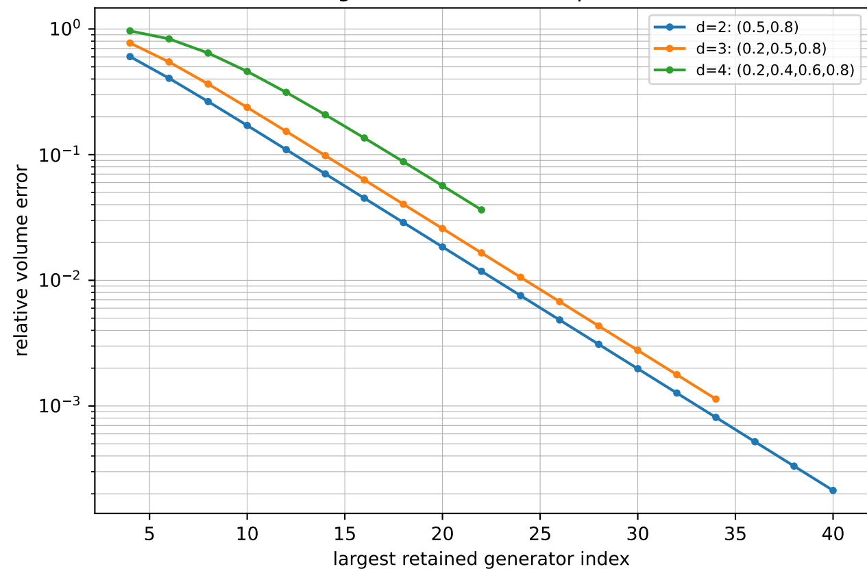
Convergence of finite zonotope volumes
