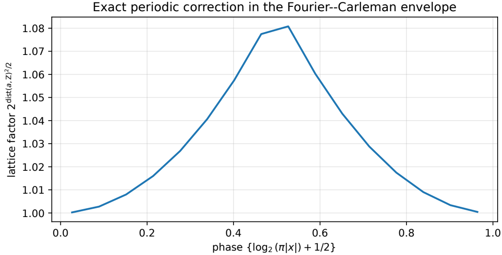
Figure 1: The exact lattice factor in (54). It is not a numerical artifact: it is the rounding cost in the discrete Legendre transform.
