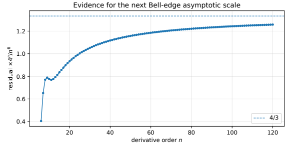
(b) Scaled residual and the conjectural 4/3 limit.
