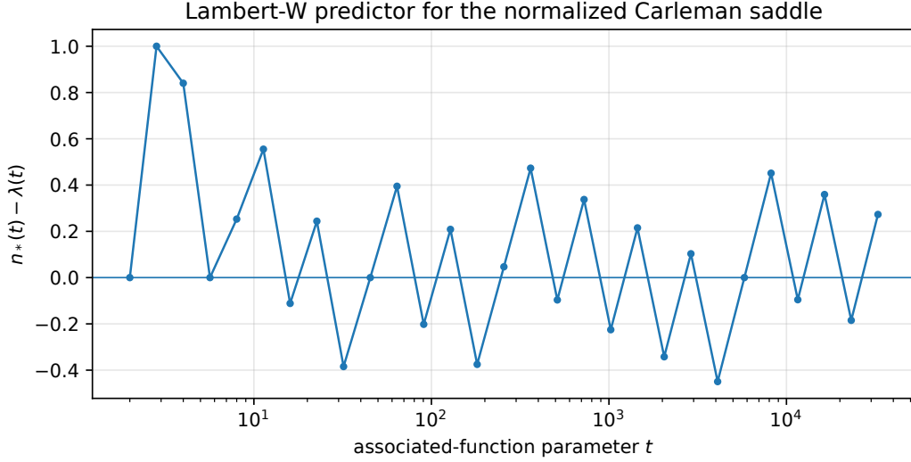
Figure 3: The exact discrete optimizer n_*(t) minus the Lambert predictor (65). Integer rounding produces the bounded sawtooth; the continuous saddle error is much smaller.
