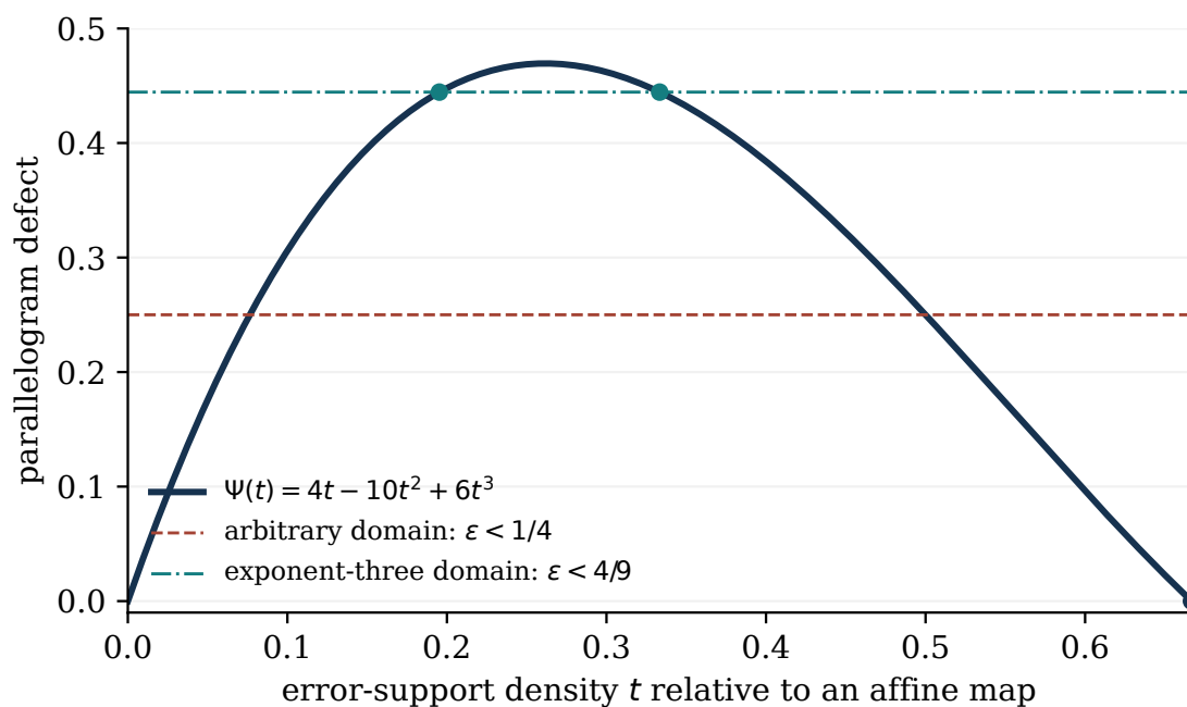
Figure II.295.1: The local cubic profile and the two strict universal recovery thresholds. The profile is relative to any affine reference and is not monotone over its full positive interval. Recovery uses its increasing branch up to \rho = (2 - \sqrt{2})/3 ; the proof excludes the intervening branch before invoking the inverse. The plot is not a claim that every point on the curve is an attainable nearest-affine extremum.
