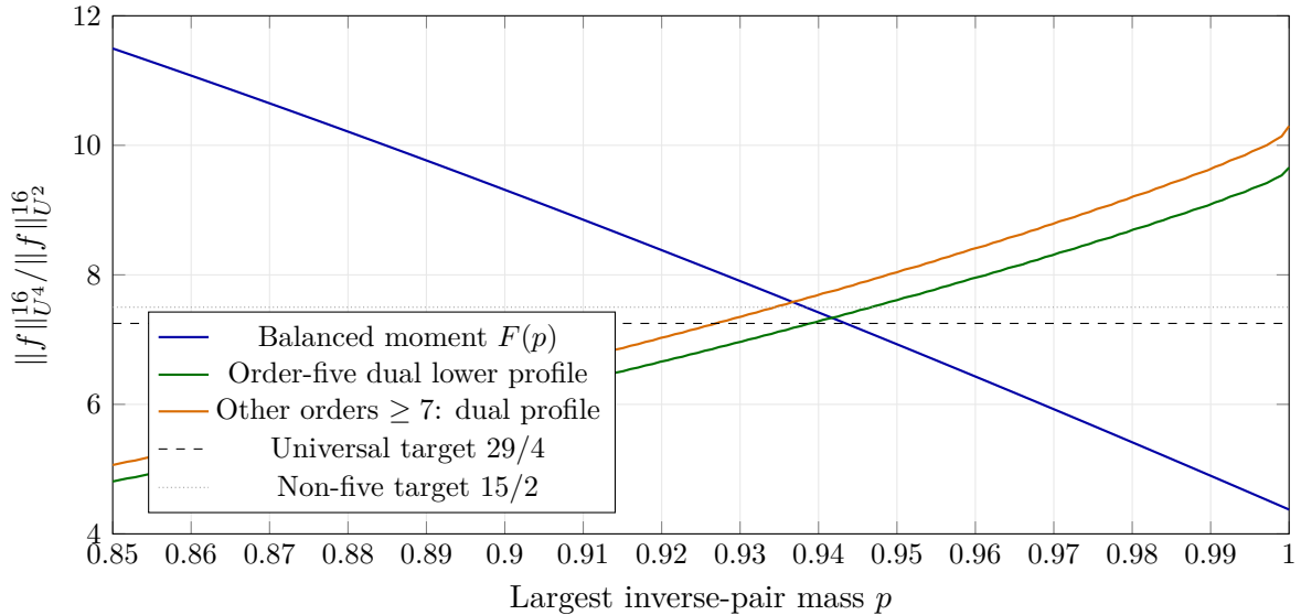
Figure III.93.1: For each applicable character order, the ratio is bounded below by the larger of its moment and dual profiles. The two estimates cover the transition region with a strict rational margin. Order three has its separate stronger projection bound.
