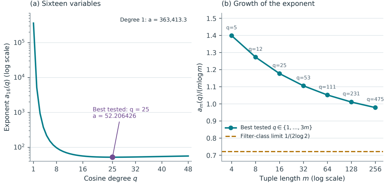
Figure V.218.1: Numerical exploration of powered cosine filters. The left panel shows the dependence on the degree at m = 16 . The right panel normalizes the best sampled exponent by m \log m . The dashed reference line is the limit for the infimum over the full filter class, 1/(2 \log 2) , proved in Theorem B. It is not a claimed limit of the degree-restricted finite search. Numerical data select candidates; the exponent-54 conclusion uses exact integer certificates.
