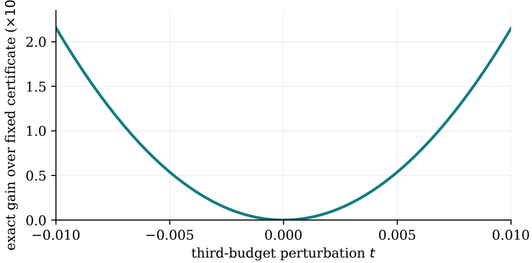
Figure I.76.1: The exact gain over the old fixed certificate in the three-frequency example, as the third budget changes by t . The plotted quantity is 96t^2/[49(91+12t)] ; the proof gives this expression exactly. The vertical scale is in millionths.
