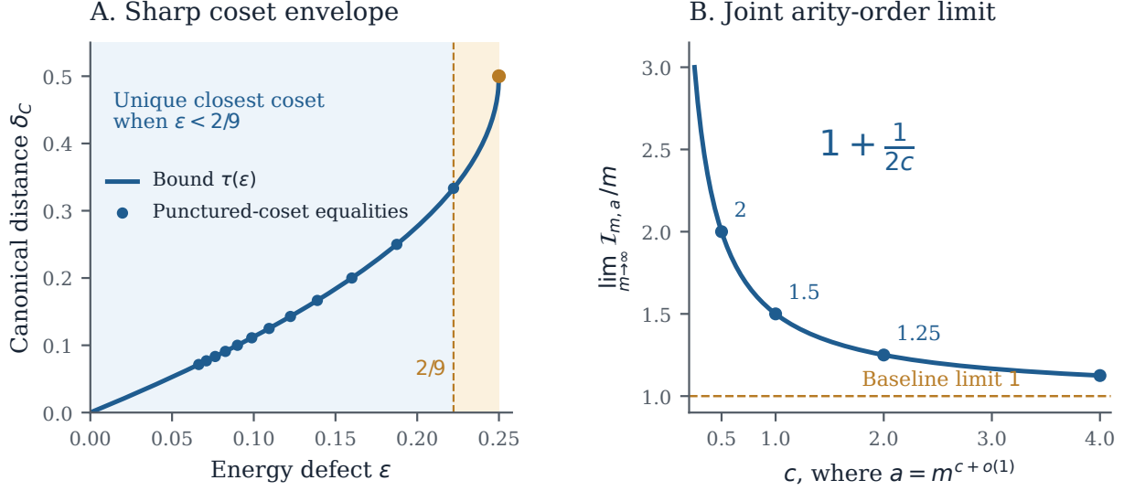
Figure F.73.1: Two proved profiles. Left: the canonical coset envelope, with punctured-coset equality parameters marked. The blue region has unique closest-coset guarantees; the remaining interval through 1/4 retains existence. Right: the asymptotic principal cost when the discrepancy order is a power of the arity. This is a limiting curve, not a finite-arity numerical estimate.
