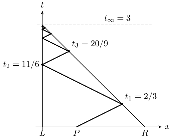
Figure 3: A four-speed accumulating clock. The drawing displays only a finite number of segments; the formulas specify all finite prefixes.
