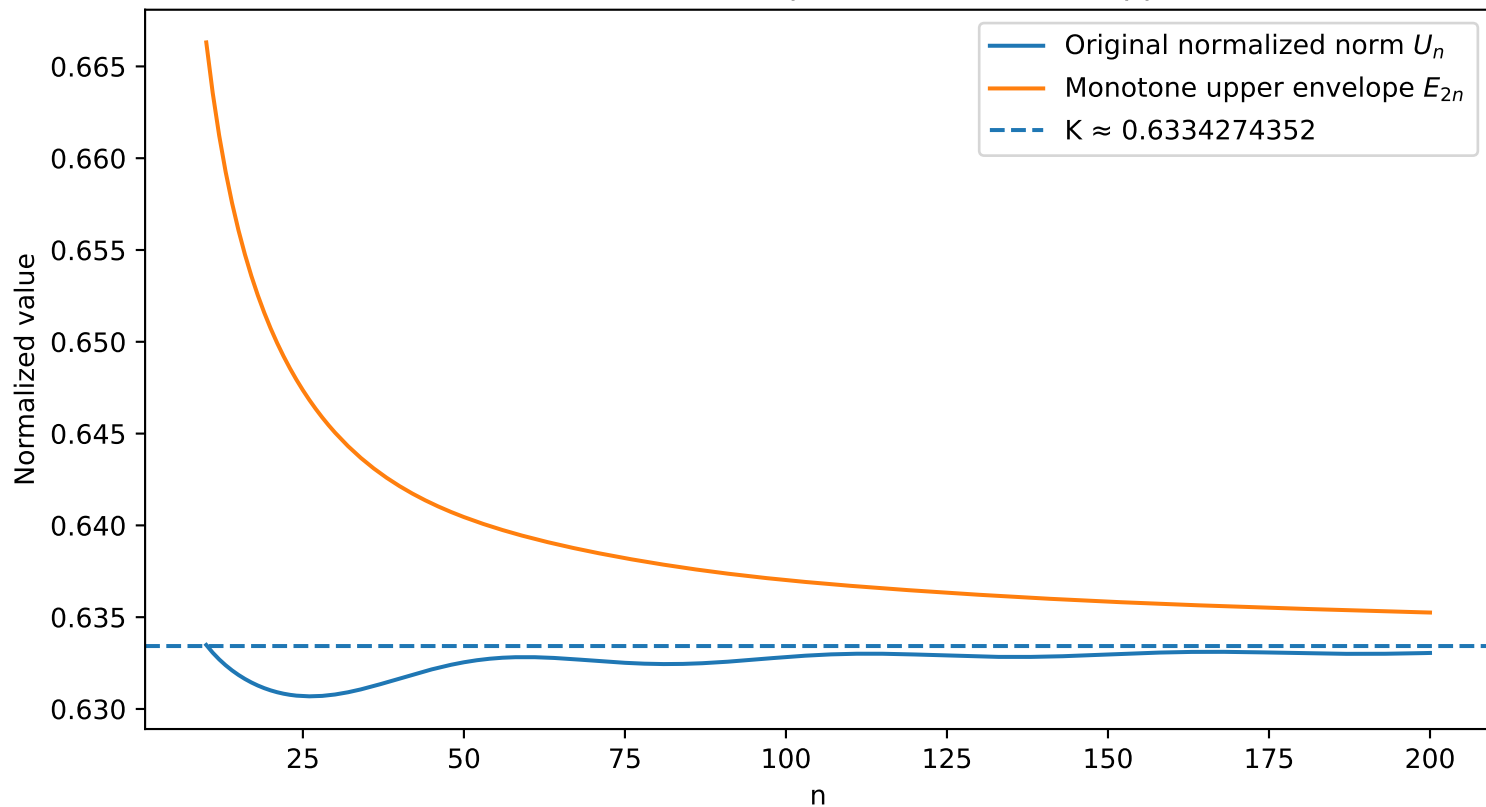
Related Hankel determinants produce monotone upper bounds
