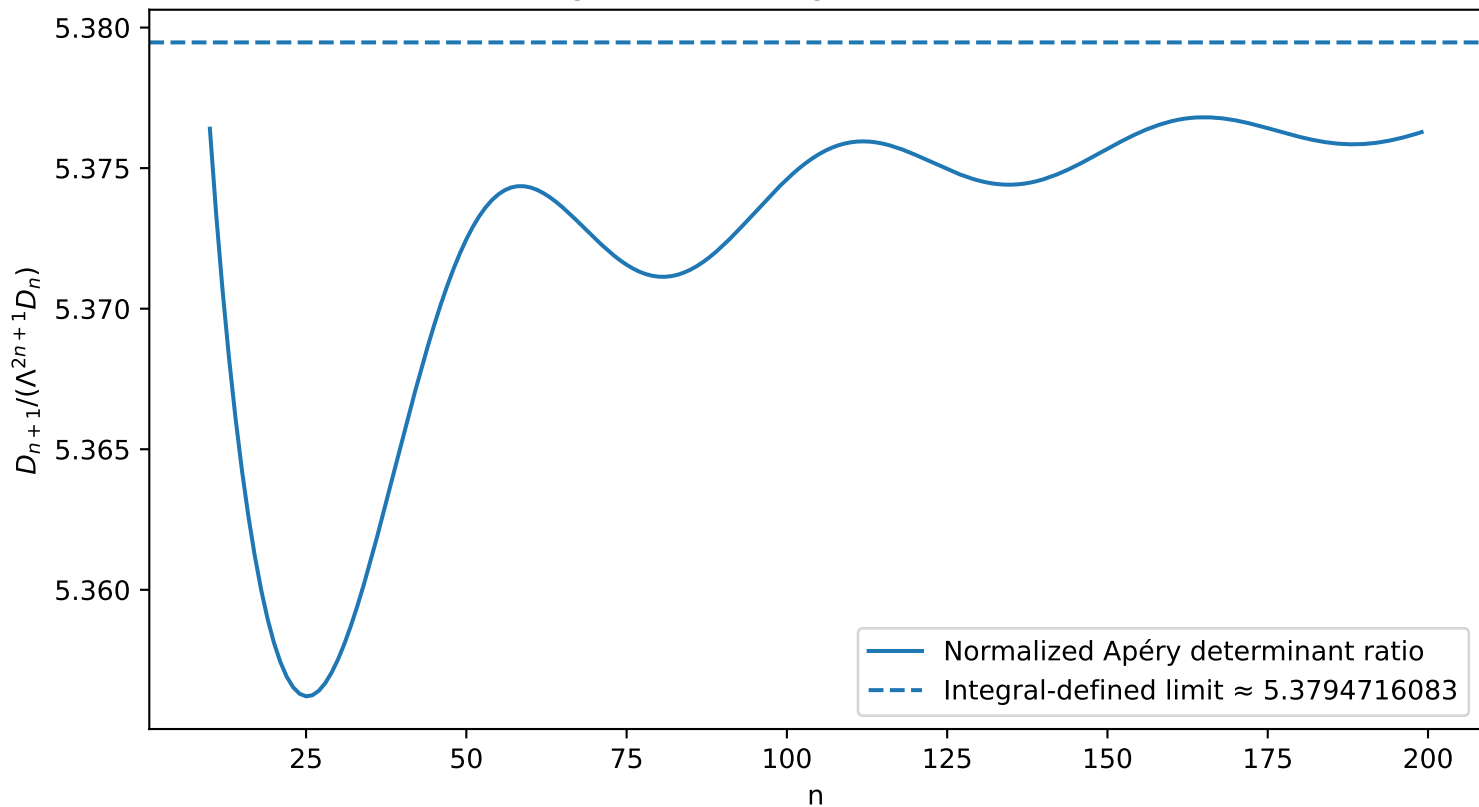
The oscillating ratios converge to a well-defined constant
