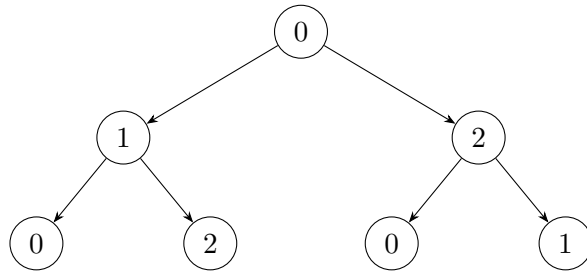
Figure 1: The finite pattern tree for example 65.2. In the actual Hausdorff forcing skeleton, each displayed child type is represented by an infinite sequence converging to its parent. The seven-point drawing is a pattern diagram, not a finite Hausdorff realization of the accumulation.
