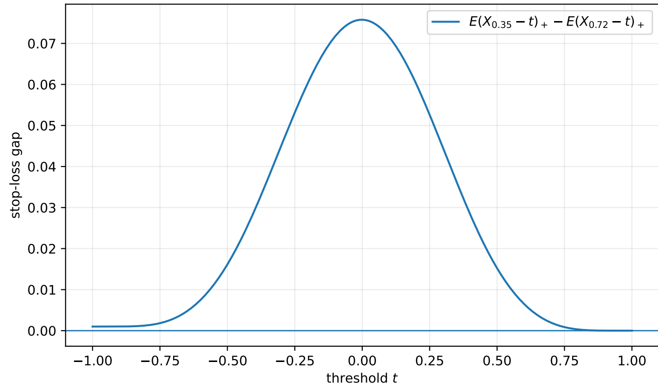
Convex-order parameter flow: empirical diagnostic
