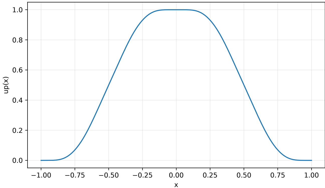
Rvachev up-density from the refinement fixed point
