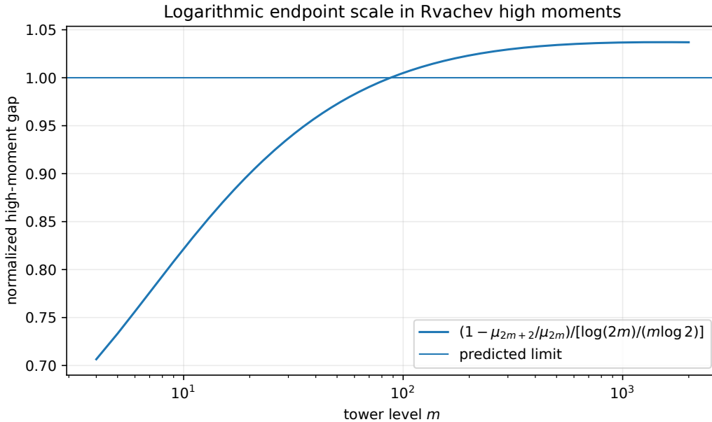
Figure 3: The normalized gap in (99), computed by the positive moment recurrence in Appendix A. The slow drift above one is consistent with the explicit constant term in (98); the periodic term is much smaller on this scale.
